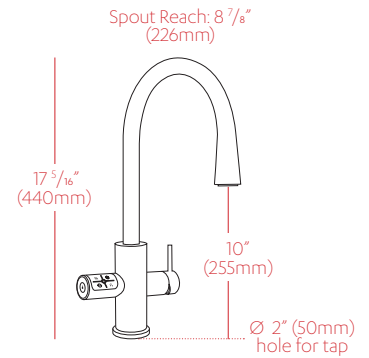
Celsius Plus All-In-One (no Pull-Down Sprayer)
