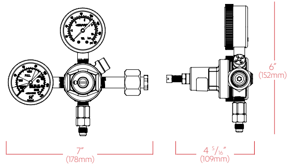
CO 2 Regulator
