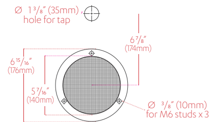
Stand Alone Design Range Font for Arc Plus and Cube Plus
