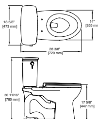
CST786CEFG.10 (Elongated)
