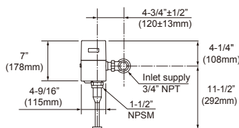
Back Spud Wall Mount 1-1/2" & 1-1/4"
