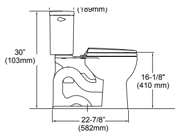
CST786CEFG.10 (Elongated)
