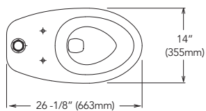
12" rough-in dimensions
