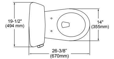
CST786CEFG.10 (Elongated)
