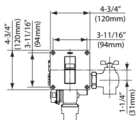
Top Spud Wall Mount 3/4"
