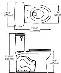
CST786CEFG.10 (Elongated)
