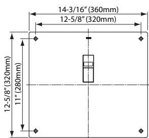
Top Spud Wall Mount 3/4"
