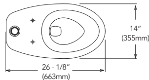
12" rough-in dimensions
