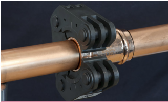
1. Fit the pressing ring
